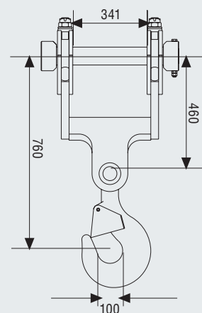
Lasthaken TLH 180
